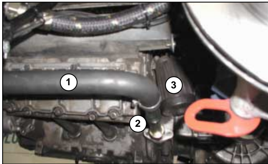
(1) S-Hose, (2) Inlet Adapter Tube, and (3) Filter
